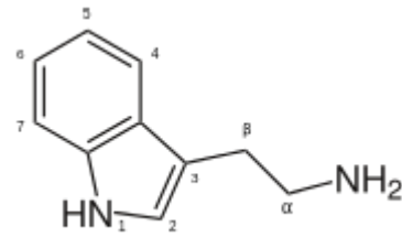
Figure 4: Squelette tryptamine
