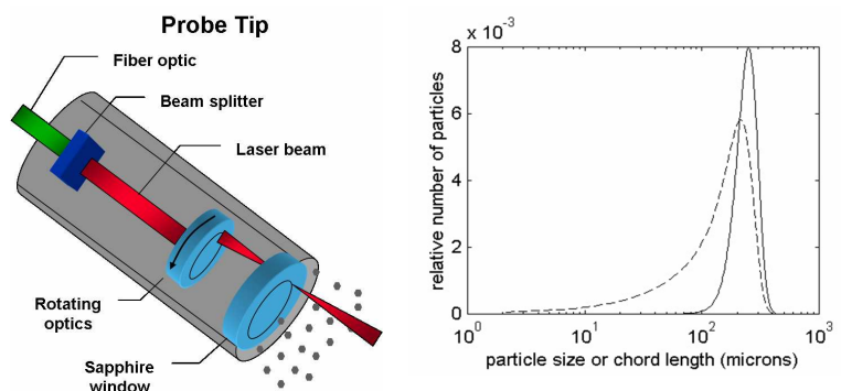
Figure 2-6 Schematic of the FBRM probe for measuring particle characteristics during process operations and Chord length distribution from FBRM (- - -) and particle size distribution (—) for polymer beads during a suspension polymerization reaction
