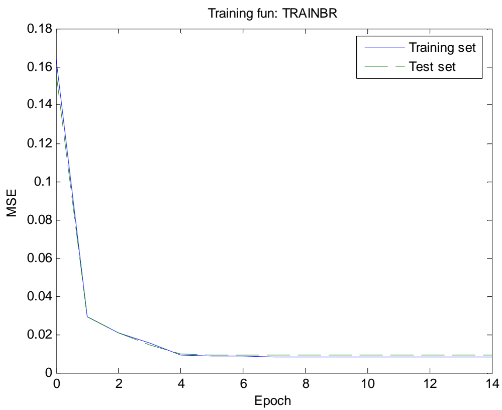
Figure 6-9 training of NN Model 2 using TRAINLM or TRAINBR
