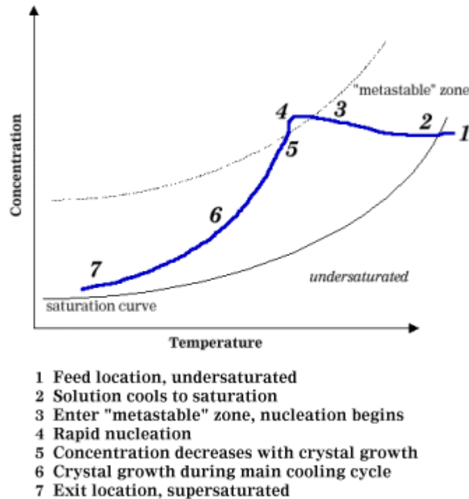
Figure 2-2: Progression of Crystallization
