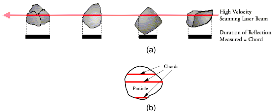
Figure 2-7 (a) High velocity scanning laser beam and duration of reflection measured-chord, (b) possibility of chord length of particle. [Source: www.lasentec.com .]
