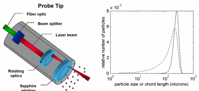
Figure 2-6 Schematic of the FBRM probe for measuring particle characteristics during process operations and Chord length distribution from FBRM (---) and particle size distribution (—) for polymer beads during a suspension polymerization reaction
