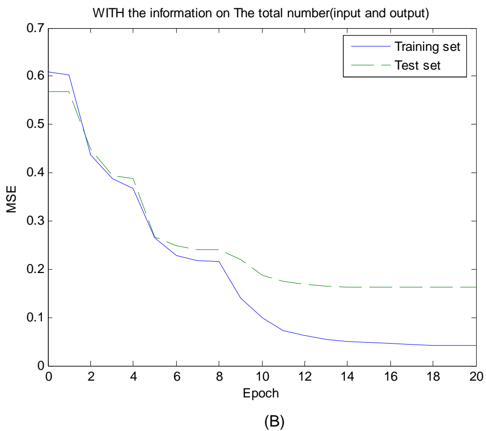
Figure 6-2 Training with TRAINLM, number of neurons in hidden layer is 11
