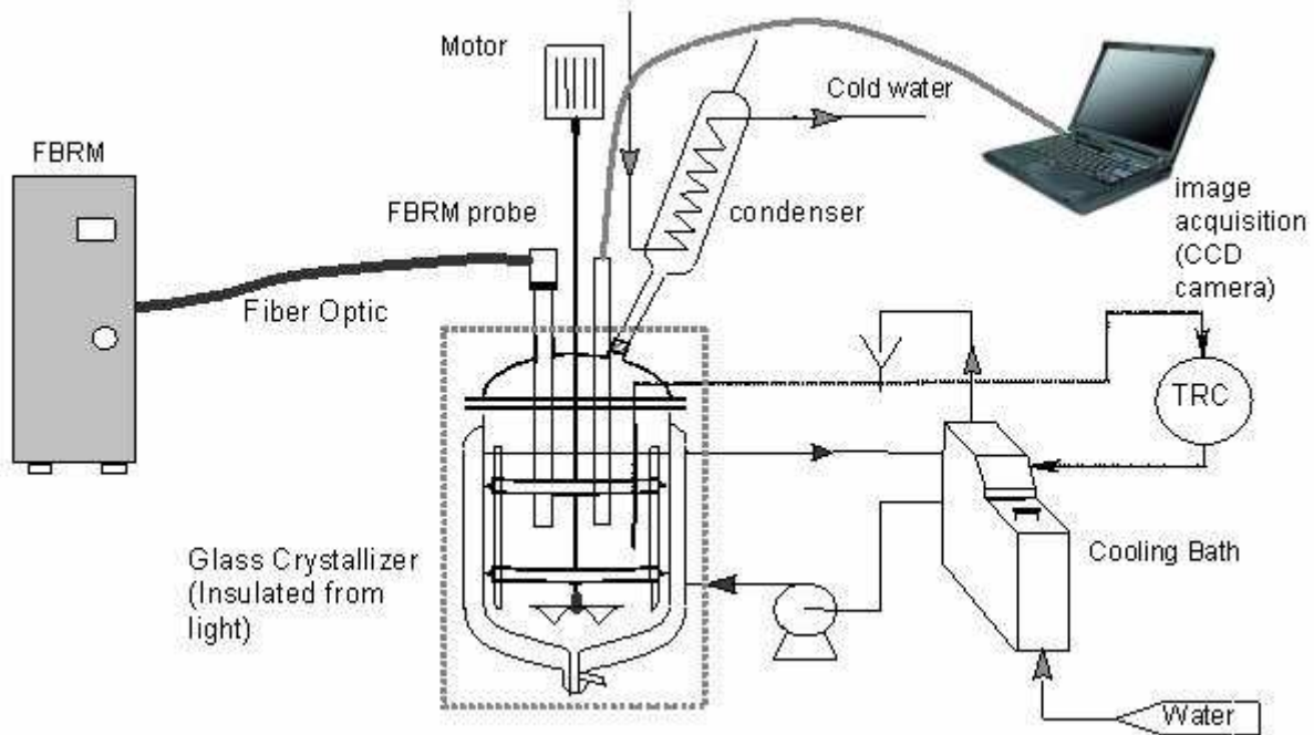
Figure 4-4 the schema of experimental equipments
