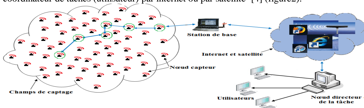
Figure 2: Architecture de communication d'un RCSF.
