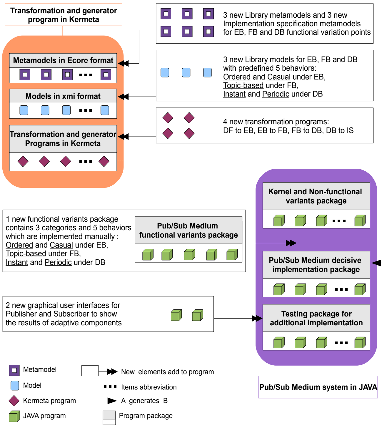
Figure 11. Prototype implementation approach and the programs relationships
