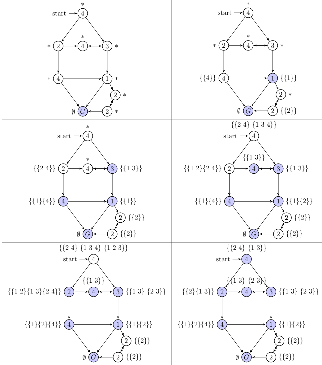
Figure 1: a trace of the executions of the pre^*_{1,3}(G) (in blue) and the position-based algorithm (the sets). Note that the positions where the coalition \{1,3\} is computed as winning are the same on both algorithms. Coalitions printed are only the smallest ones, every bigger coalitions are winning
