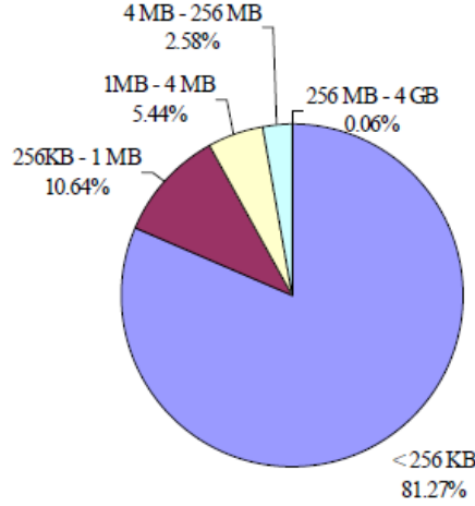
Figure 2: Package size distribution
