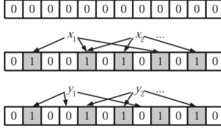
Figure 9: Example of Bloom filter
