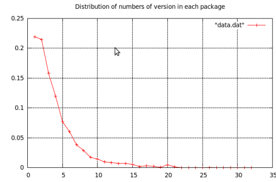
Figure 4: Distribution of numbers of version of Debian packages
