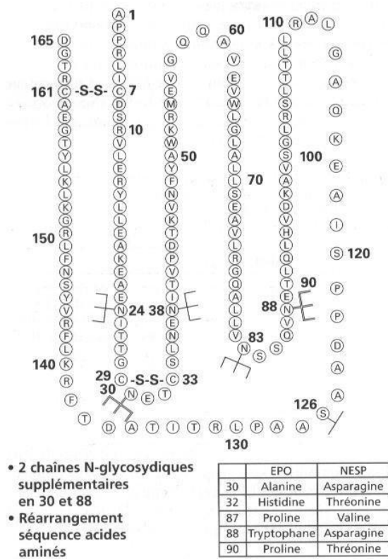
Figure 4 : Structure chimique la darbepoietin 57 (NESP)
