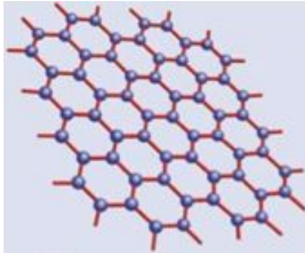
Figure 6: Graphene sheet
