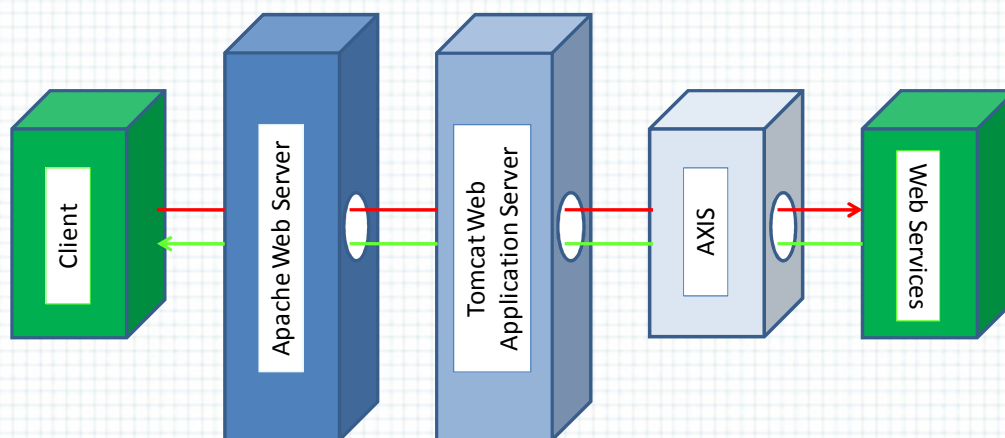
Figure 2 - L'architecture Apache
