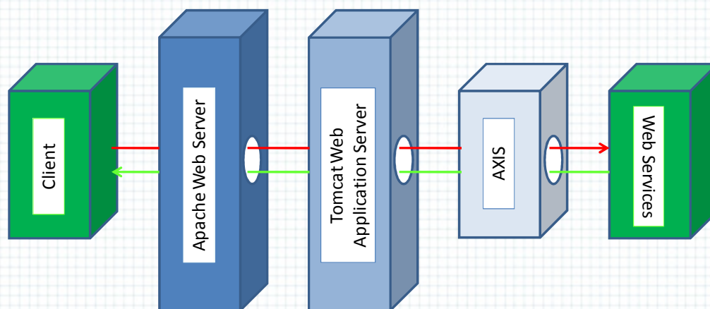
Figure 2 - L'architecture Apache
