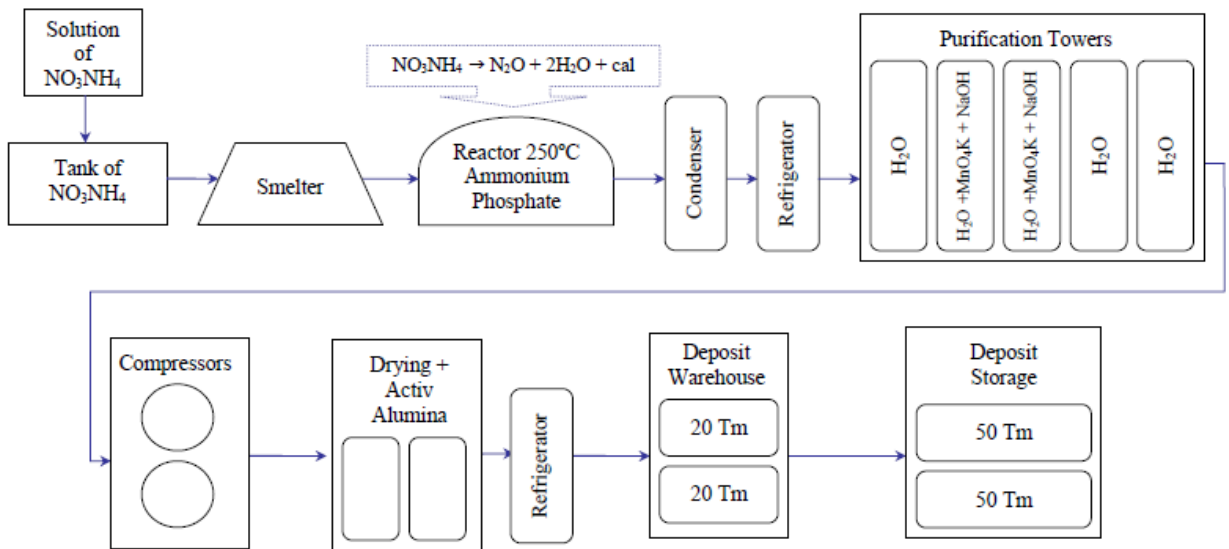
NITROUS OXIDE Diagram of production process
