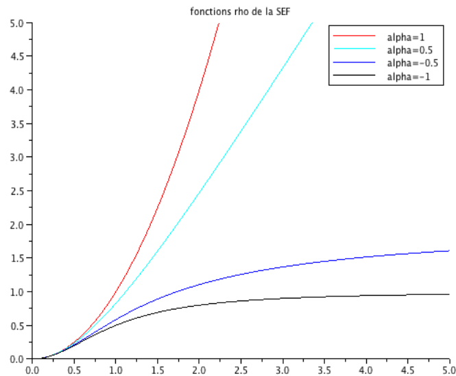
FIGURE A.2 – Smooth Exponential Family
