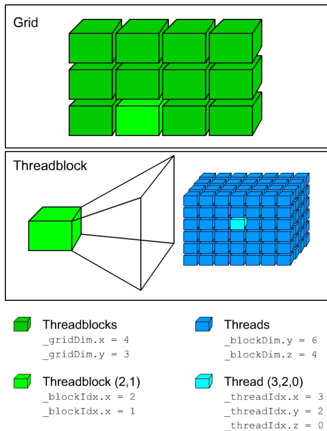
Figure 11: CUDA architecture (with arbitrary values as an example)
