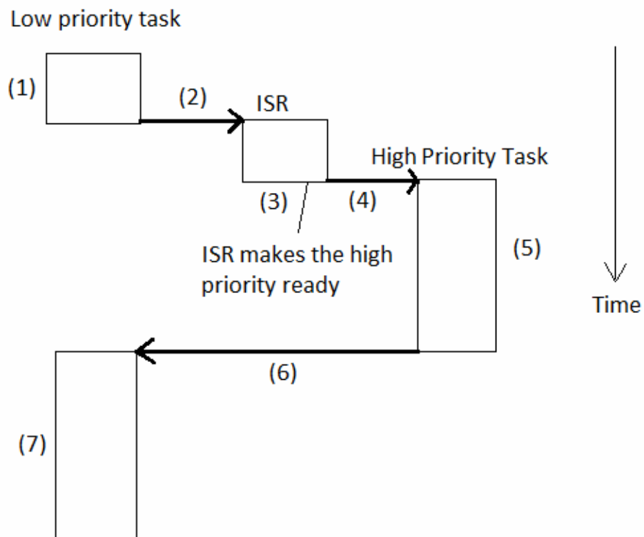
Figure 2.9. The way a preemptive kernel works [18]
