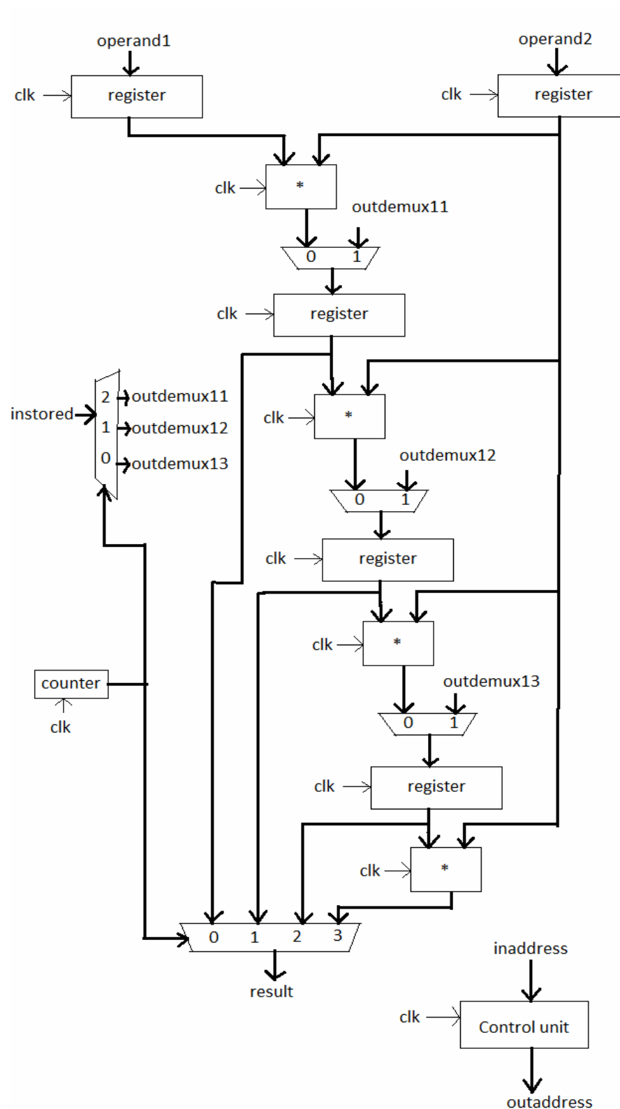
Figure 5.5. Hardware architecture of the hardware task that contains a hierarchy of multipliers
