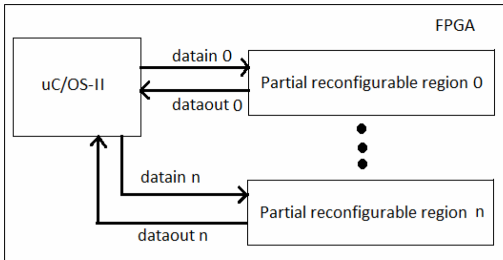
Figure 4.1. The top view of the system
