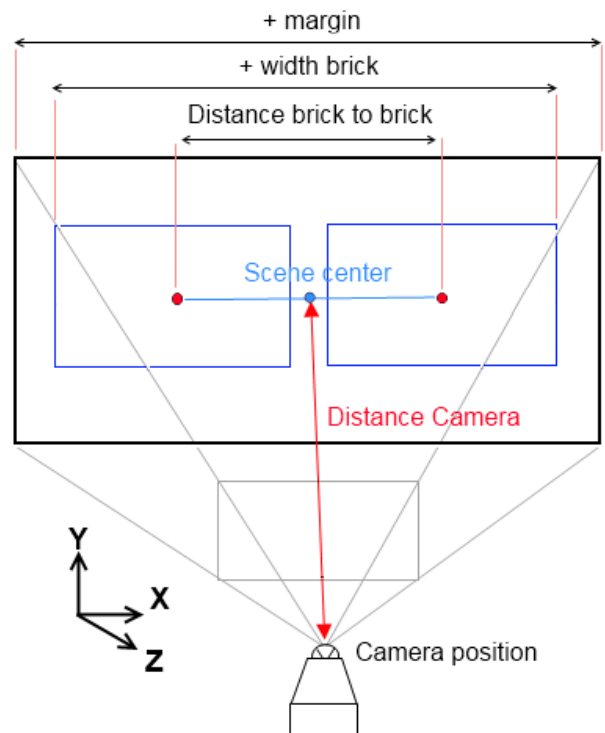
Figure 4.4: Algorithm and scheme of camera positioning
