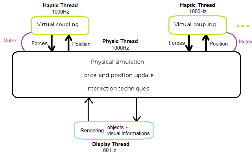
Figure 3.2: Organization of the haptic interface framework
