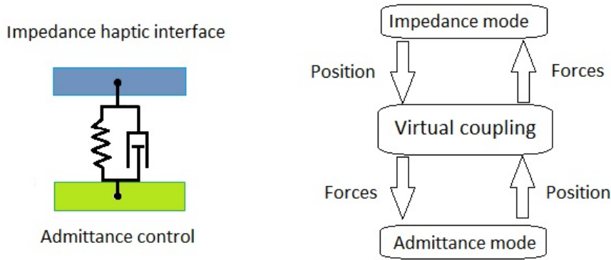
Figure 3.3: Virtual coupling spring and damper
