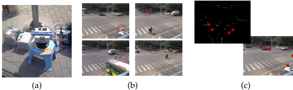
Figure 10: (a) A stand alone laser scanner. (b) A target box is placed at different places in the intersection. (c) The box is used as a calibration target to register all the lasers within a common frame.
