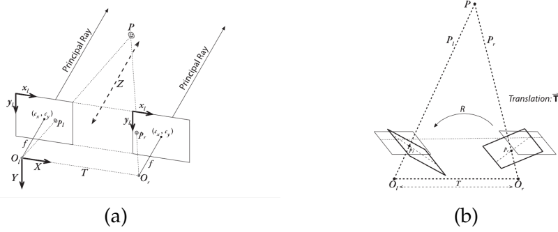
Figure 14: (a) Ideal stereo cameras system. (b) Actual uncalibrated stereo system. The image is taken from [4].
