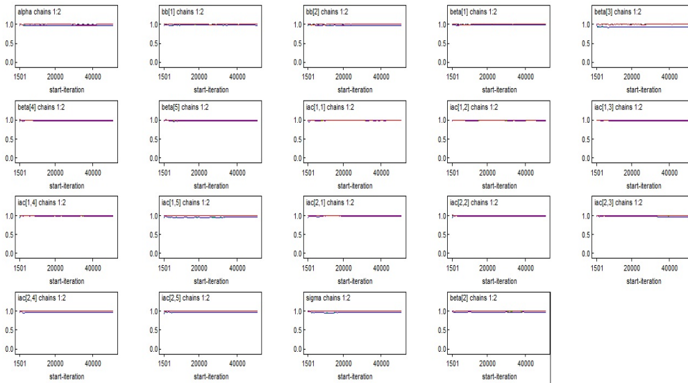
FIGURE C.2: Diagnostic de Gelman et Rubin
