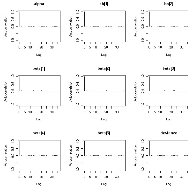
FIGURE C.1: Autocorrélation
