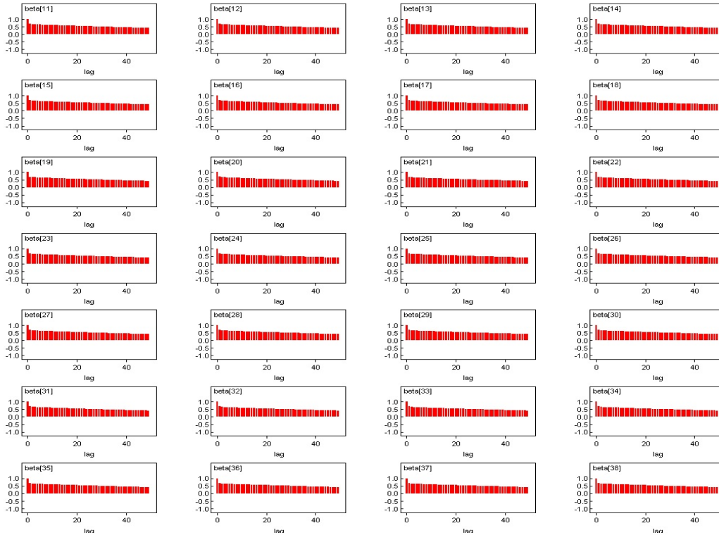
FIGURE C.3: Autocorrélations
