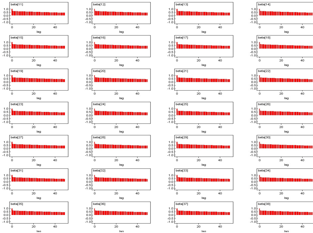
FIGURE C.3: Autocorrélations
