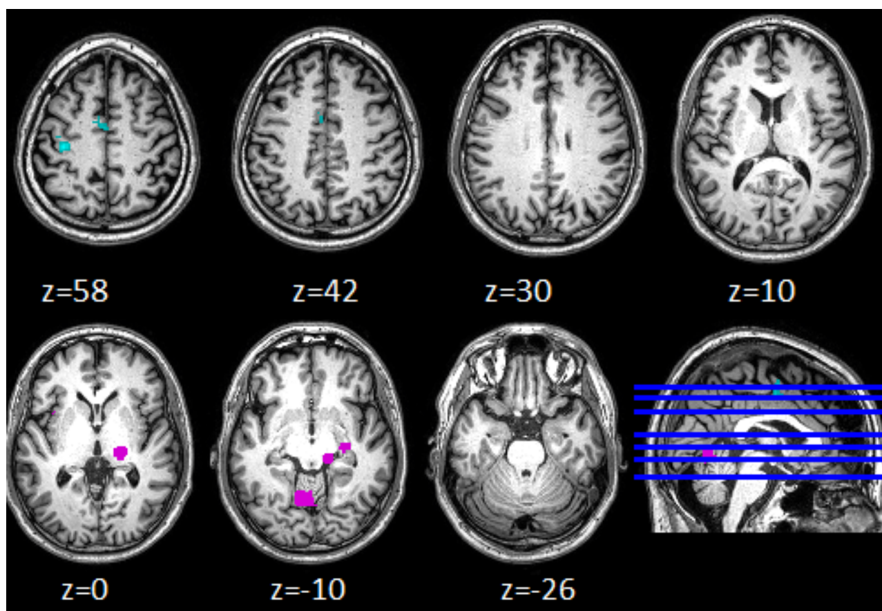
C. Comparison of ALE maxima between good (cyan) and bad (pink) outcome in chronic stage stroke patients.
