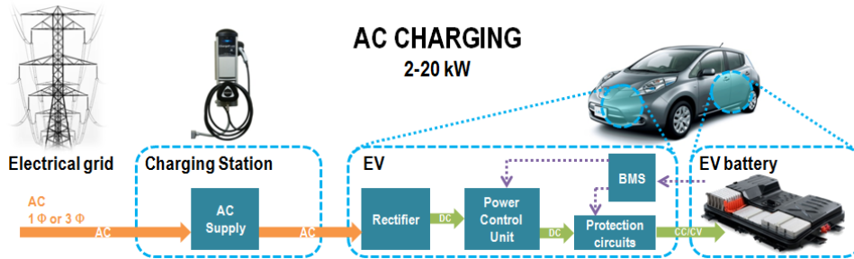
Figure 1: Schema of the AC charging process of an electric vehicle.
