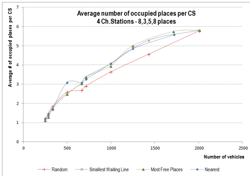
Figure 13: Average number of occupied places per charging station in function of the number of vehicles in the system for the four criteria analyzed.
