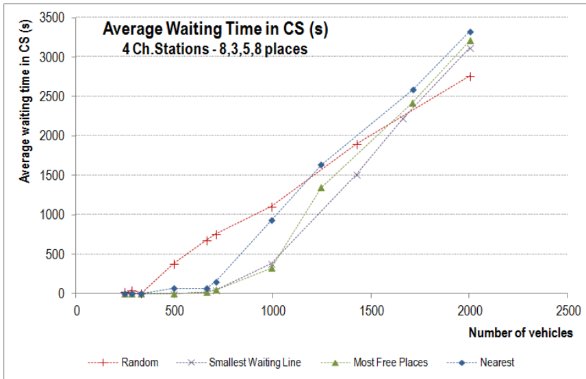
Figure 17: Evolution of the average waiting time of the electric vehicles for each one of the four strategies, in function of the number of vehicles.
