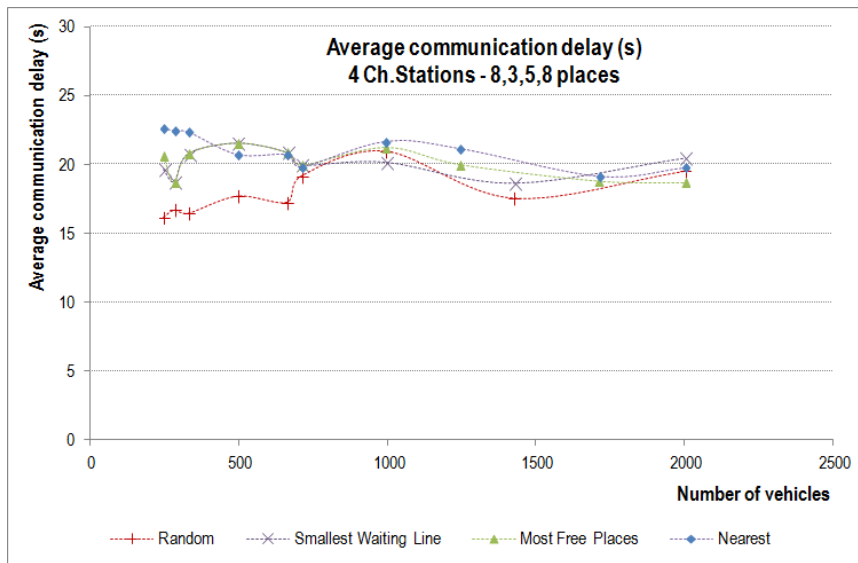
Figure 11: Average communication delay in function of the number of vehicles. Comparison between different assignment criteria.
