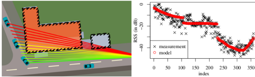
Figure 8: Evolution of the received signal strength: results obtained with the chosen path loss and obstacle shadowing models compared to experimental measurements. Source: [15]
