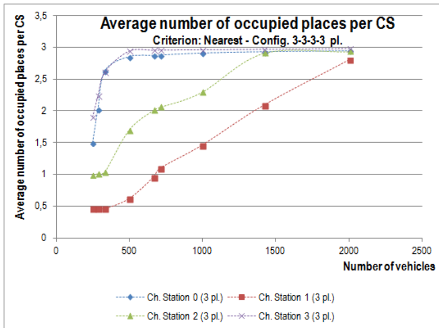
Figure 14: Individual average number of occupied places for each charging station in function of the number of vehicles in the system for the 12-place configuration.
