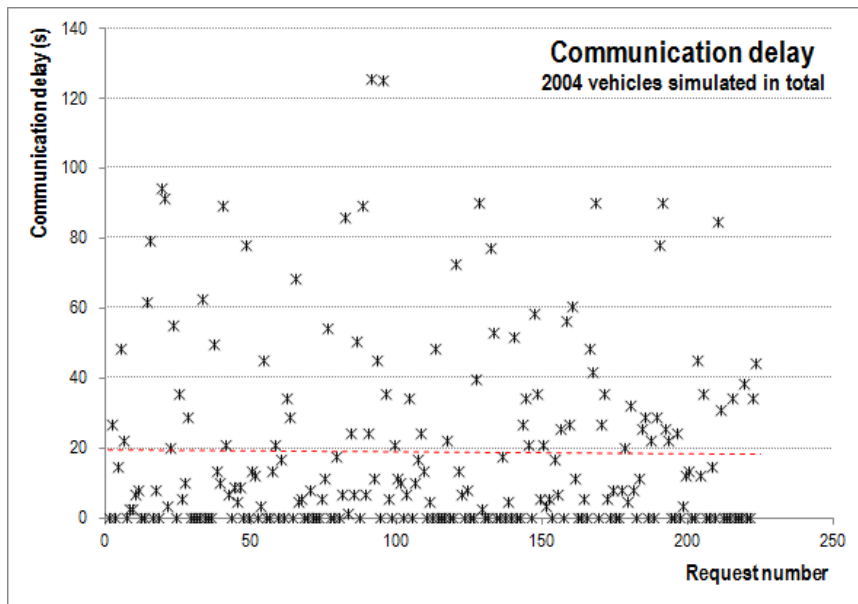
Figure 12: Communication delay for individual vehicles in a single simulation of 2004 vehicles.
