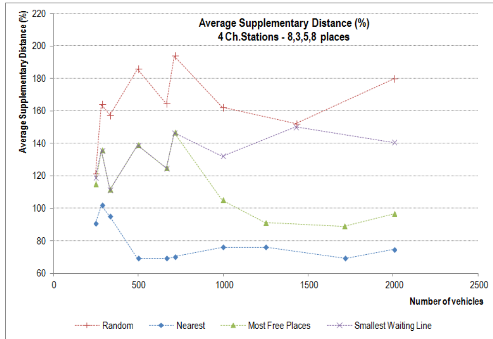
Figure 9: Average supplementary distance percentage in function of the number of vehicles in the simulation. Comparison between the four different criteria.
