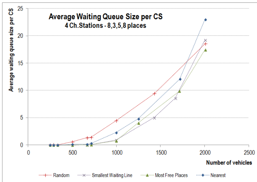
Figure 16: Evolution of the average waiting queue size per charging station for each one of the four strategies, in function of the number of vehicles.
