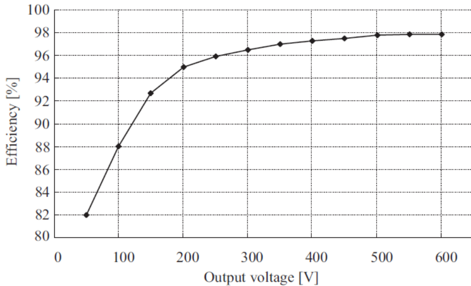
Figure 3: Efficiency in function of output voltage in a particular implementation of a DC fast charger. Source: [1]
