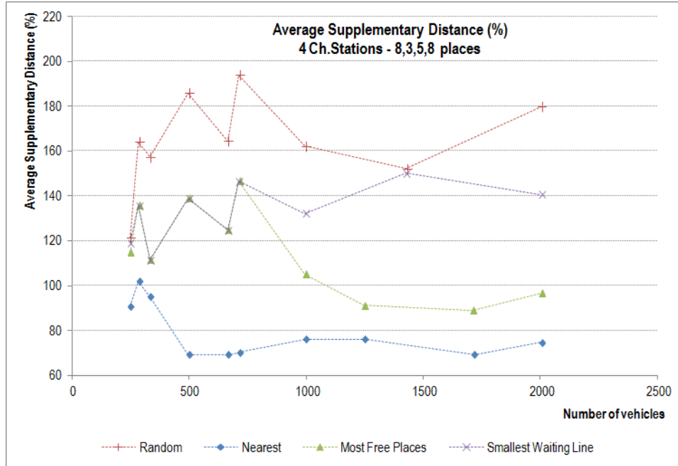
Figure 9: Average supplementary distance percentage in function of the number of vehicles in the simulation. Comparison between the four different criteria.
