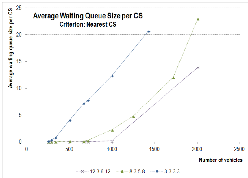
Figure 18: Evolution of the average waiting queue size per charging station for the different dimensioning possibilities, in function of the number of vehicles.
