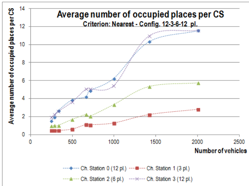
Figure 15: Individual average number of occupied places for each charging station in function of the number of vehicles in the system for the 33-place configuration.
