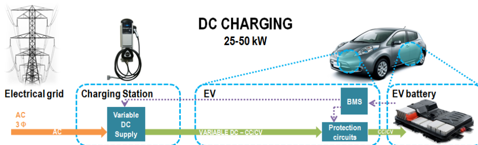
Figure 2: Schema of the DC charging process of an electric vehicle.
