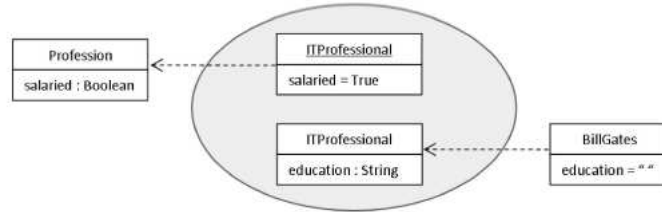
Figure 4: Facets type/instance of one concept [8]
