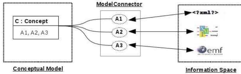
Figure 16: A concept aggregates three Abstract Elements
