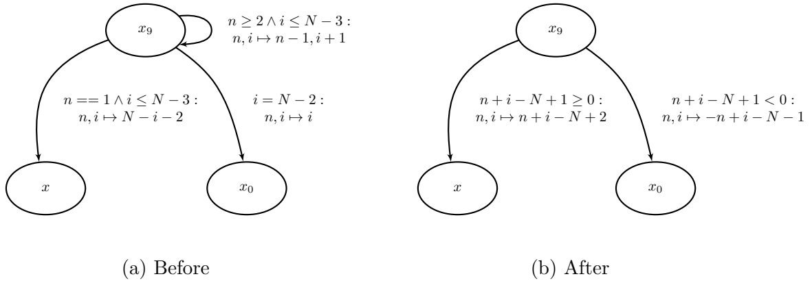
Figure 4.8: Copy relation before and after cycle elimination.
