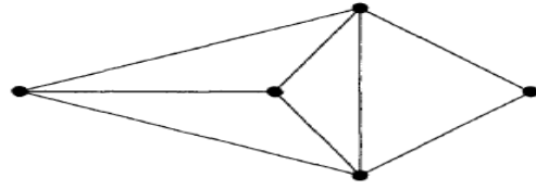
Figure 7: Isomorph graph-2
