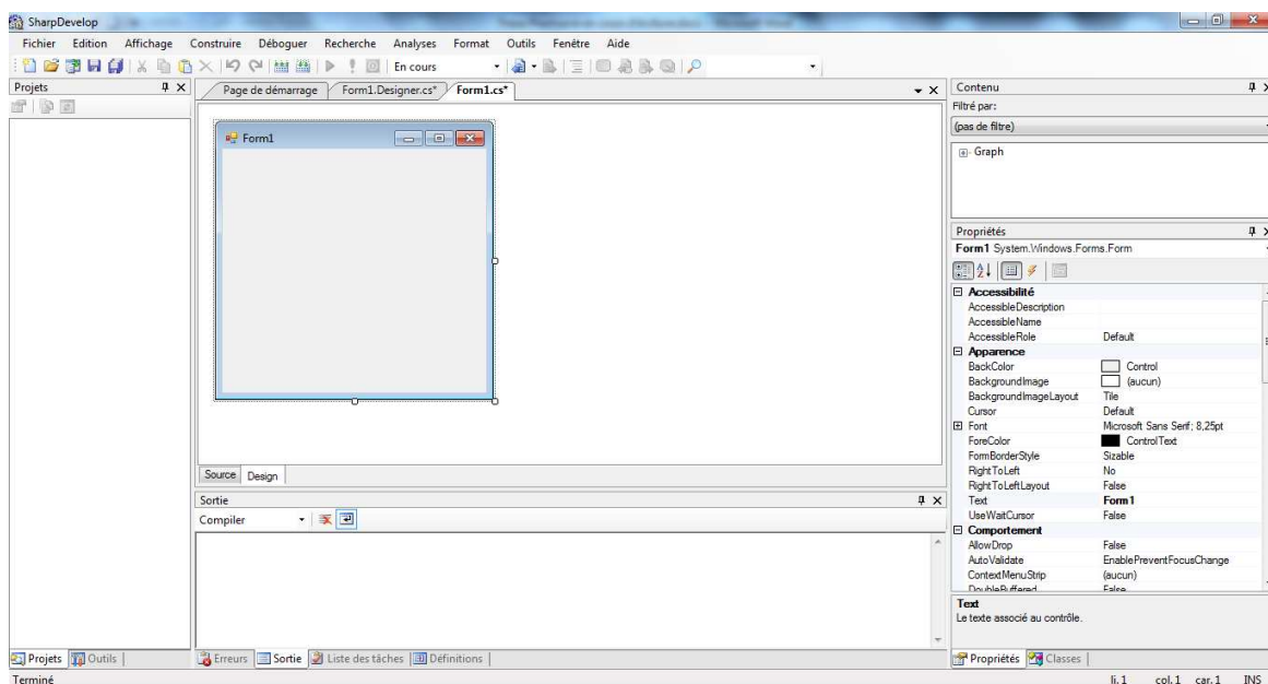
Figure 2 : Interface SharpDevelop
