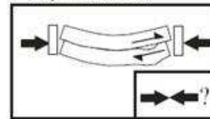
2) EW shortening and bending (Stephan et al., 1986)
