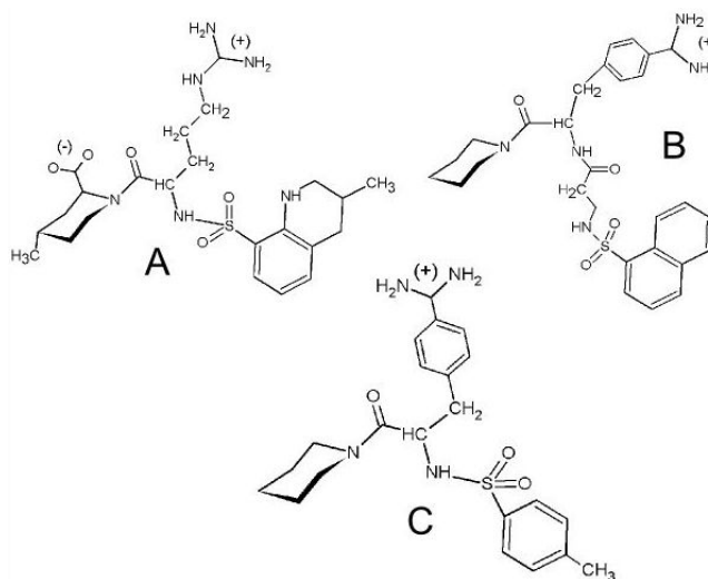
FIGURE 1.17 – Structure plane des molécules d'anticoagulant MQPA (A), NAPAP (B) et 4-TAPAP (C).
