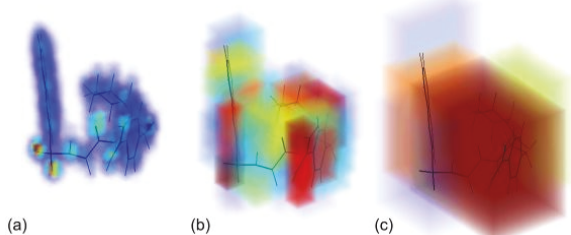
Figure 7: 3-D NAPAP EDM (resolution 120 \times 98 \times 85 ) with 5, 3 and 2 levels of TSLVQ ( Z_3 , b_2 ), respectively.
