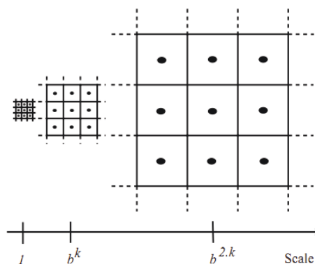
Figure 2: Hierarchical set corresponding to the cubic lattice. Here, the scaling factor b=3 [8].
