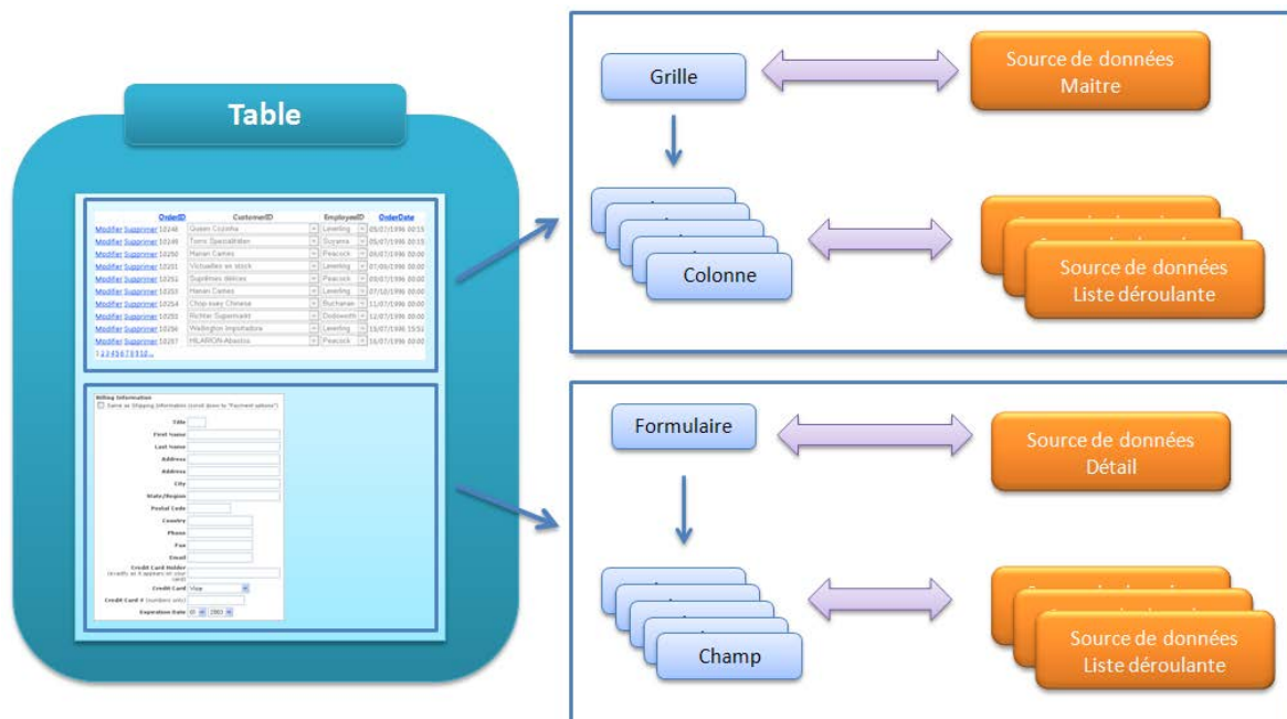
Figure 58 - Architecture du composant graphique
