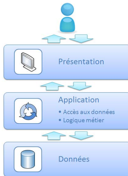
Figure 6 - Architecture 3-tiers
