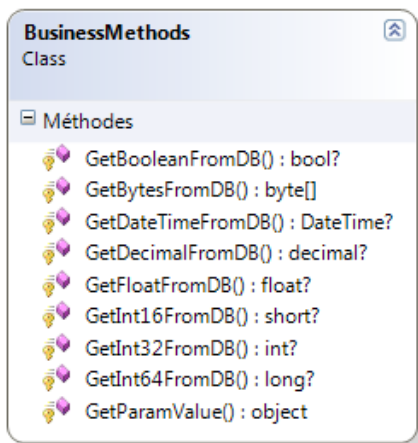
Figure 54 - Diagramme de classes BusinessMethods
