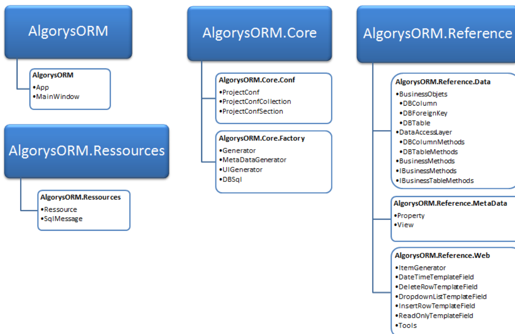
Figure 45 - Architecture logique des modules AlgorysORM
