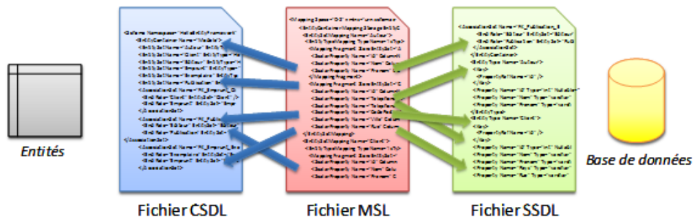
Figure 17 - Architecture Entity Data Model 4
