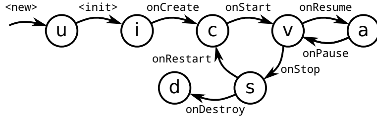
Figure 7: Definition of \mathbf{Lifecycle} \in \mathcal{P}(\mathbf{ActivityState} \times \mathbf{Method} \times \mathbf{ActivityState}) as an automata. (s, m, s') \in \mathbf{Lifecycle} means that there is a transition from state s to state s' by calling a.m() where a is the activity on which the transition applies.
