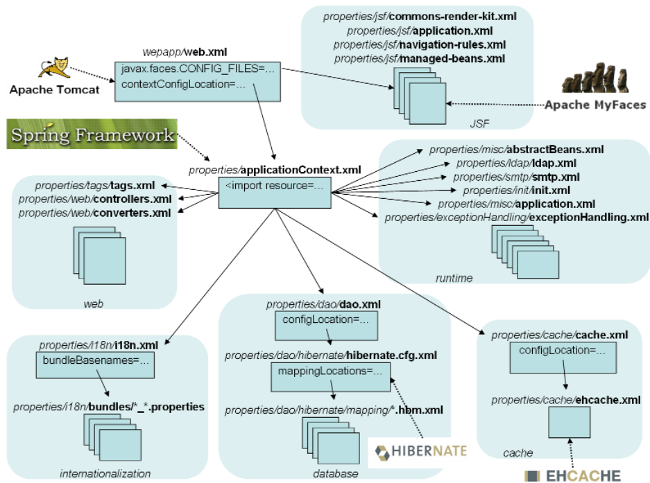
Figure 72 Configuration d'Esup-Commons
