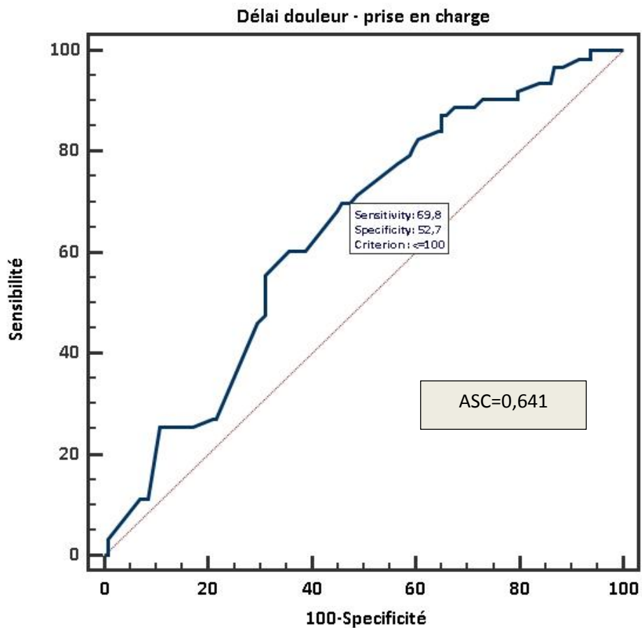
Figure 13 : Courbe ROC
