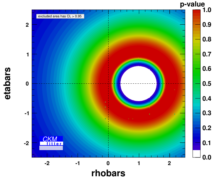
Figure 2.1: Fit of \bar{\rho}_s, \bar{\eta}_s using |V_{cb}| , |V_{cs}| and B(B_s \rightarrow \mu\mu) as inputs.
