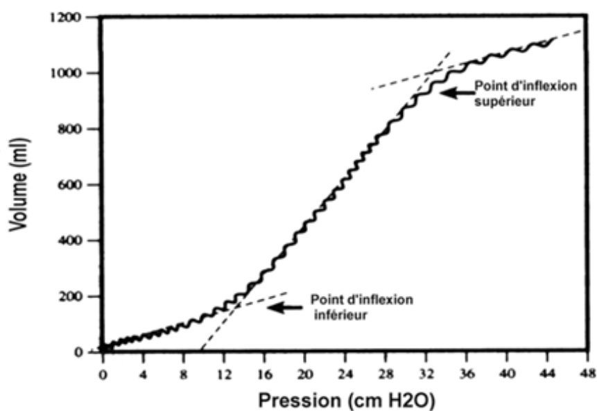
Figure n°14 : Courbe Pression/Volume [102]
