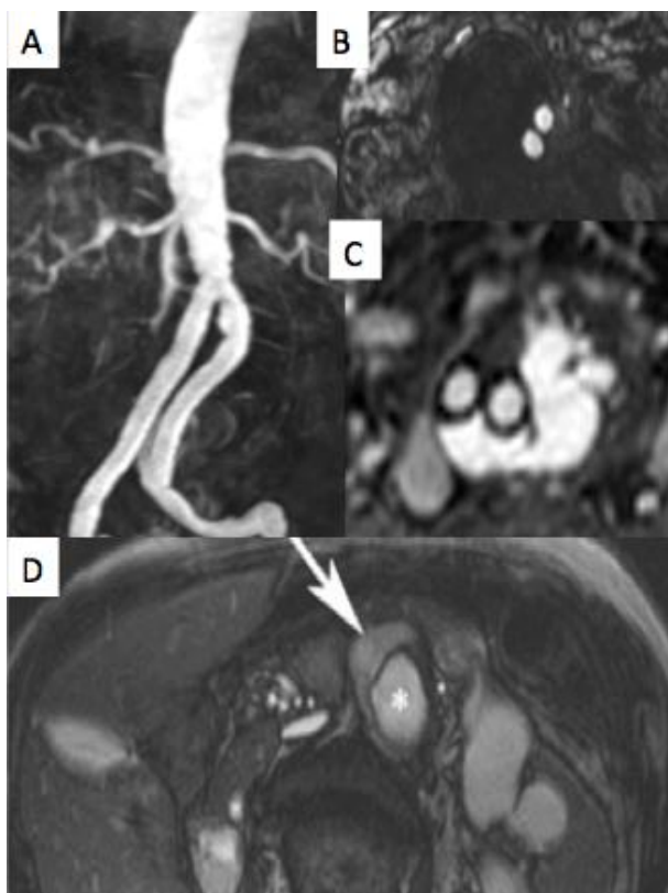
Figure 16- IRM.
