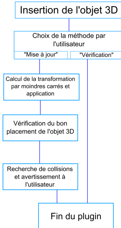
Figure 51 : Algorithme final
