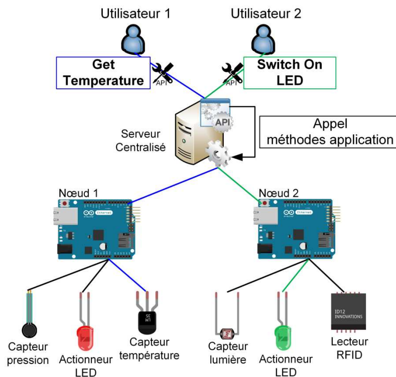
Figure 8 - API
