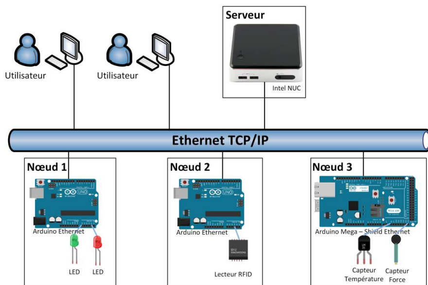
Figure 33 - Architecture matérielle
