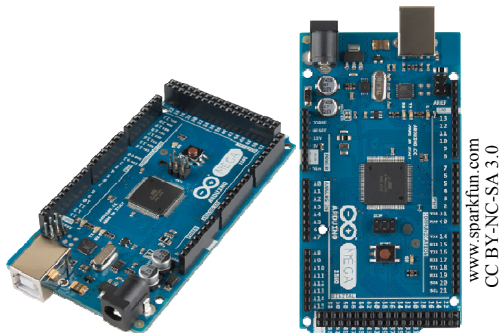
Figure 30 - Arduino Mega
