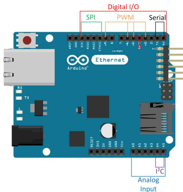
Figure 29 - Interfaces Arduino Ethernet
