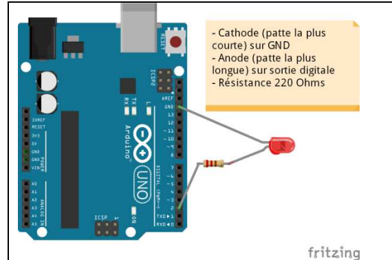
LED
