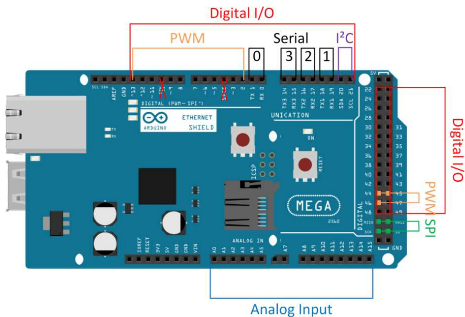
Figure 31 - Interfaces Arduino Mega et shield Ethernet
