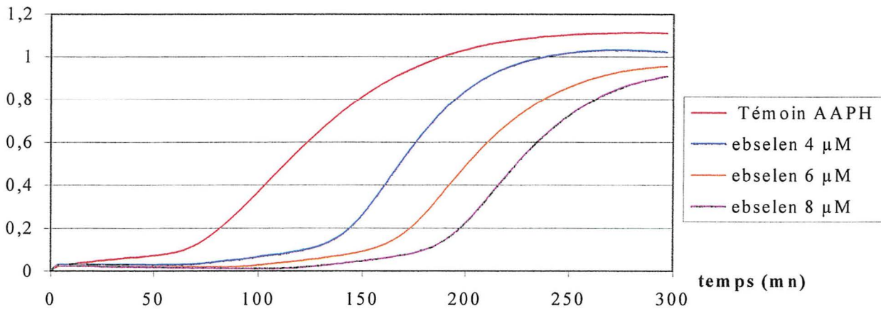
figure 5c: ebselen et AAPH
