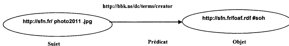
Figure 9: Triplet RDF
