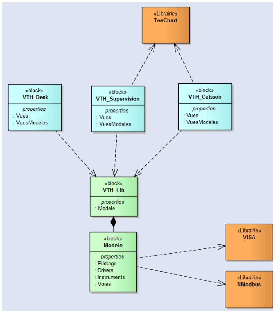
Figure 24 Architecture technique
