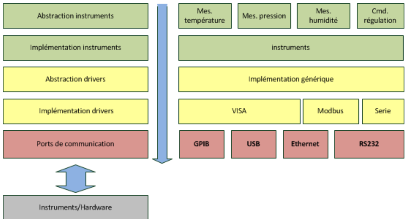
Figure 27 Architecture du composant instrument
