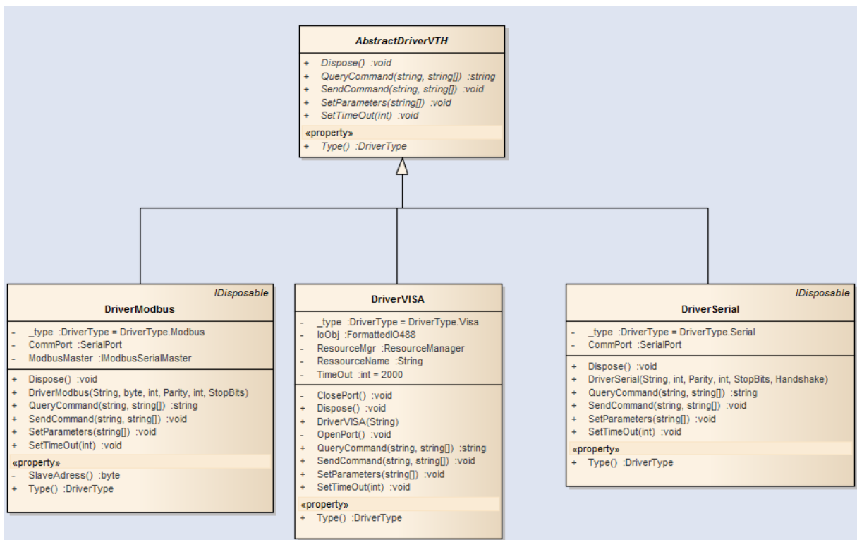
Figure 28 Classes couches drivers
