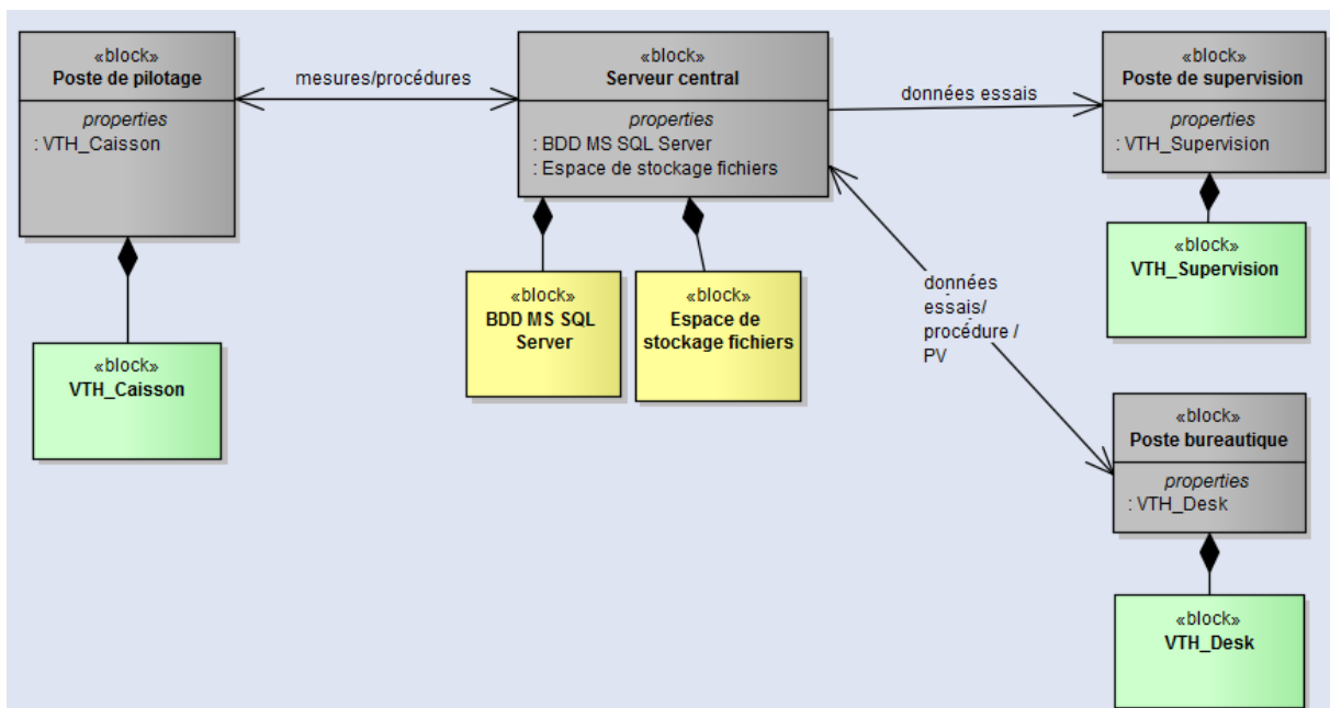
Figure 25 Architecture physique
