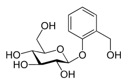
Salicyline
