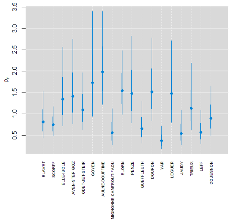
Figure 3.2. Multiplicative effects of years (left) and rivers (right)
