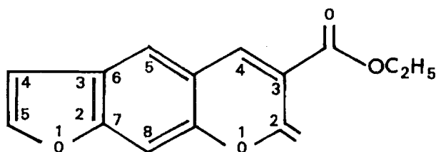
3-carbéthoxypsoralène
