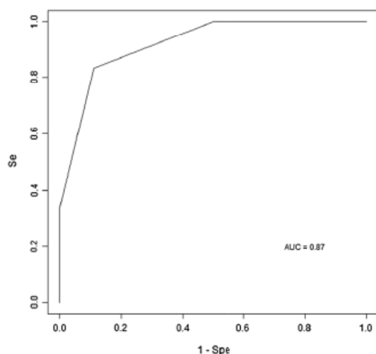
Fig. 3 ROC curve
