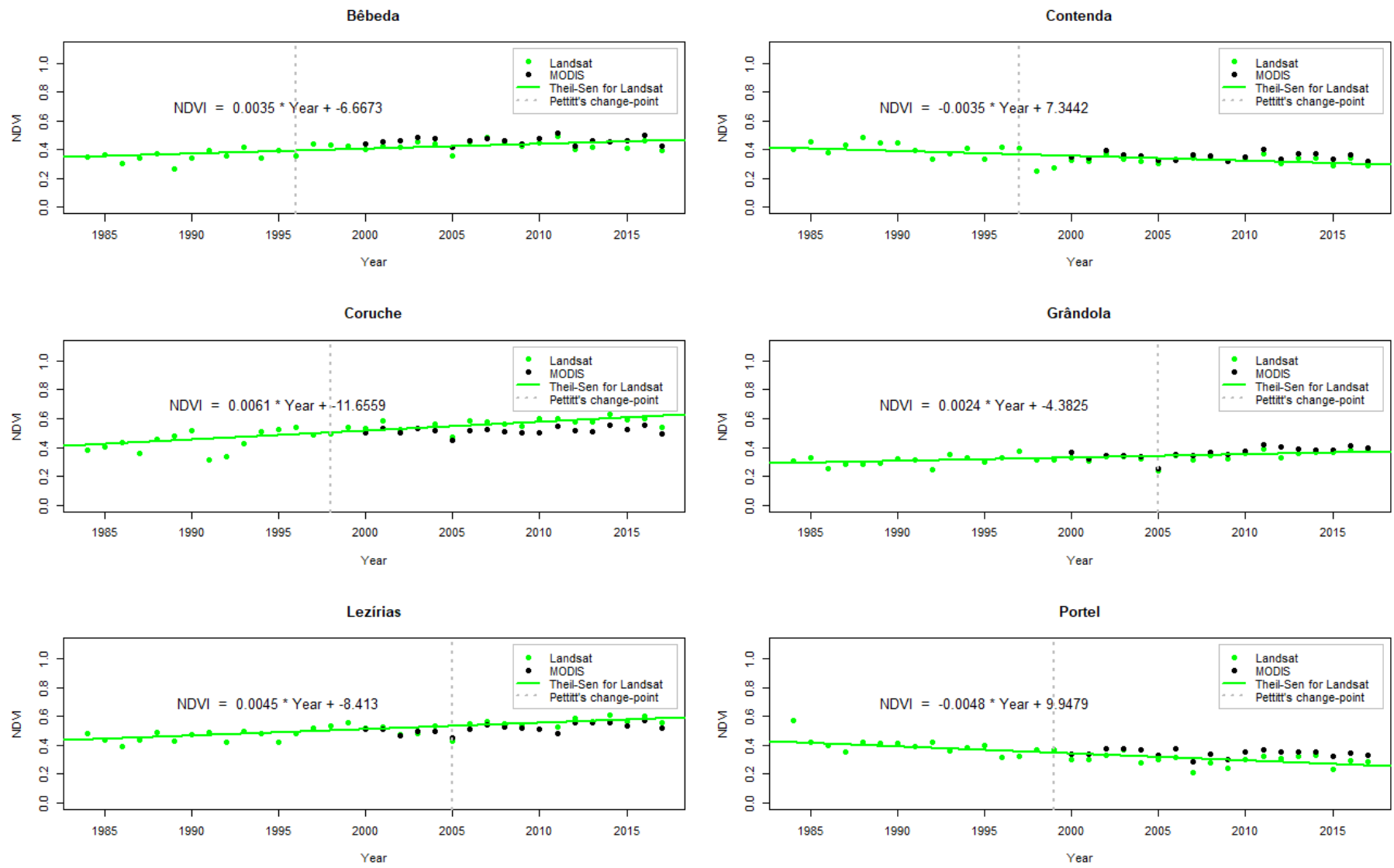
Figure 6: Landsat NDVI summer means per year for each study-site.
