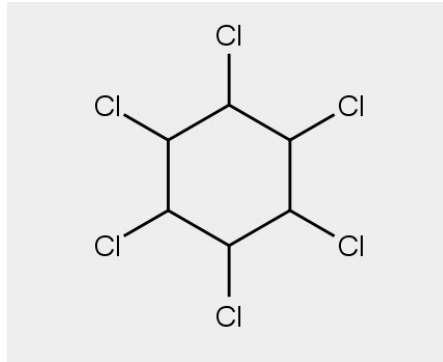
Figure 52 : lindane
