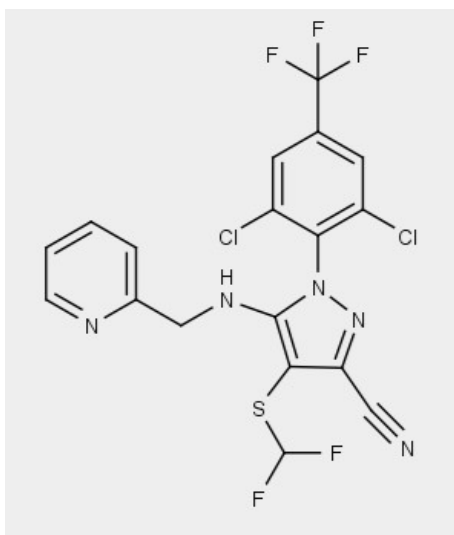
Figure 58 : le pyriprole
