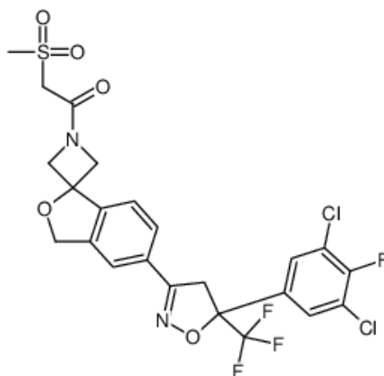
Figure 69 : le sarolaner
