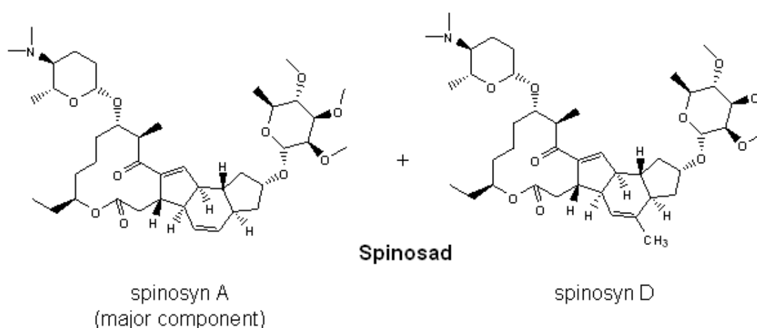
Figure 67 : le spinosad
