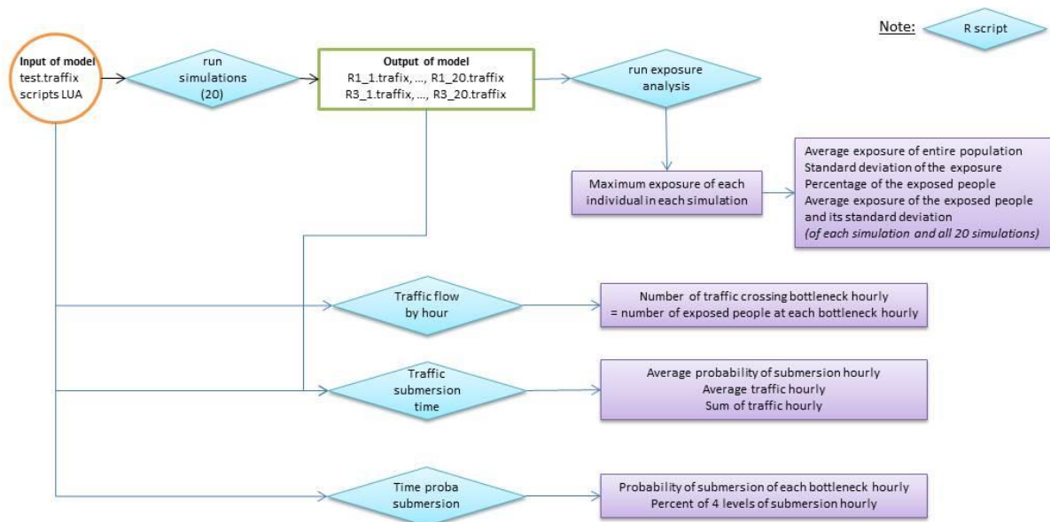
Figure 8: Calculation scheme
