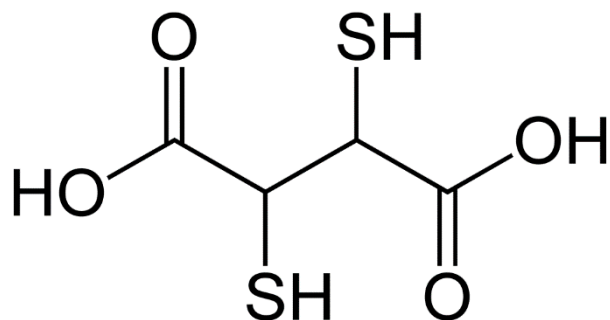
Figure 12: DMSA
