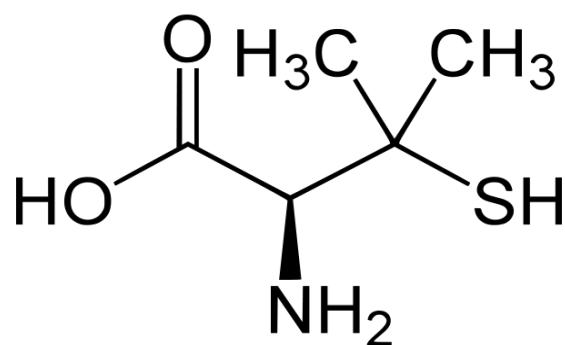
Figure 10: D-Pénicillamine
