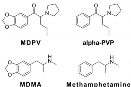
Fig. 1. Molecular structures of MDPV, α-PVP, MDMA and Methamphetamine.
