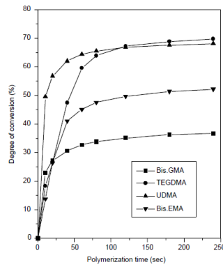
Fig. 1. Degree of conversion of C = C double bonds (%) as a function of irradiation time, for the neat dimethacrylates. The solid lines are calculated fits of the experimental data to the Eq. (1).
